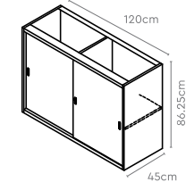
VSDU-10 (with Metal Top)
