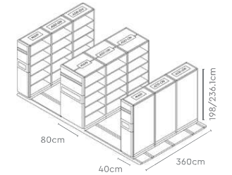
M3 Motorized with Platform
